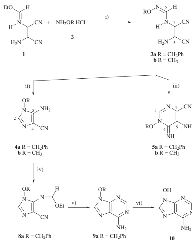
Scheme 1 Reagents and conditions: i, EtOH, RT, 2 h–2 days; ii, NaOH, EtOH, RT; iii, DBU, ¼ equiv.; ethyl acetate, RT; iv, Ac 2 O, CH(OEt) 3 , reflux, 16 h; v, NH 3 (aq), MeOH, RT, 2 h; vi, HBr 32% in AcOH, steam bath, 3.5 h.
