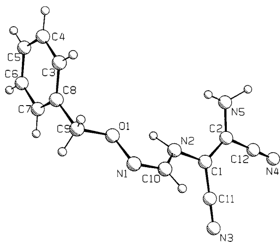
Fig. 1 X-Ray crystal structure of ( Z )- N -(2-amino-1,2-dicyanovinyl)formamide O -benzyloxime 3a .
